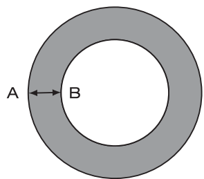
Bushing cross section: The entire bushing wall is hardened (from point A to B)
