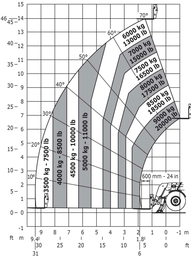
Rotation on lowered stabilisers with forks - CoG 600 mm
